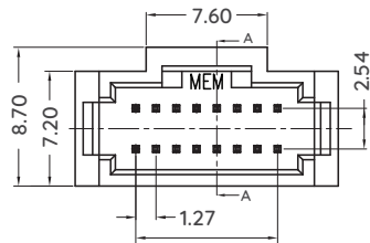
1.27 X (No. of Ways in One Row -1)
