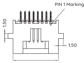
1.27 X (No. of Ways in One Row -1)+4.60
