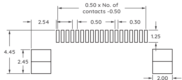
RECOMMENDED P.C.B LAYOUT (PCB BOARD TOLERANCE ±0.05)
