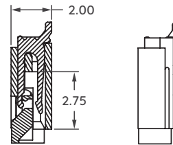
SECTION A
