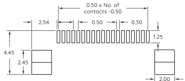
RECOMMENDED P.C.B LAYOUT (PCB BOARD TOLERANCE \pm 0.05 )
